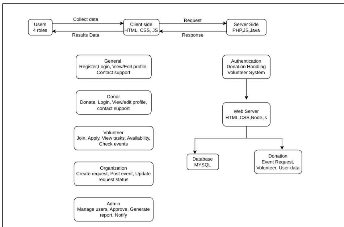
Figure 4: System Architecture
