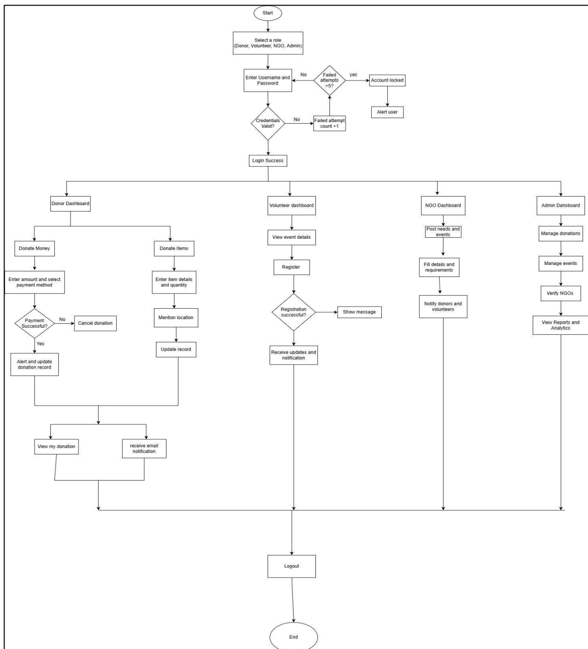
Figure 3: Flowchart
